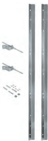
38562001 Rapid SL set for corner installation 2 wall brackets 1.13m for WC, bidet, wash basin and urinal
